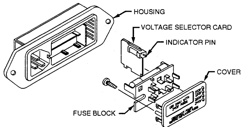
Figure 2-13. Line Voltage Selection (A)
