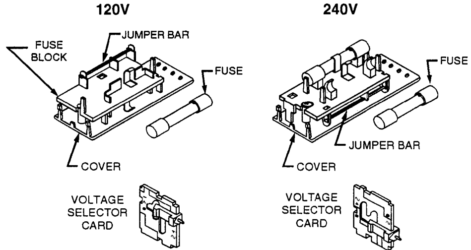
Figure 2-14. Line Voltage Selection (B)
