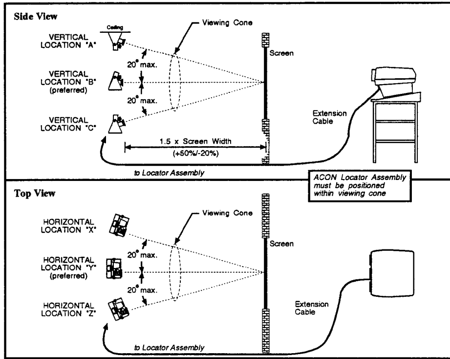
Figure 2-23. Remote Locator Assembly Placement
