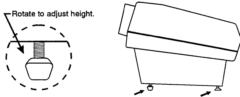
Figure 2-8. Leg Adjustment
