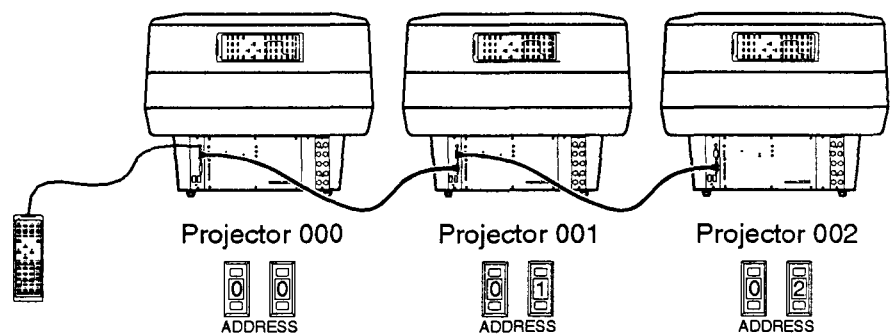
Figure 2-18. Wired Remote Control of Multiple Projectors
