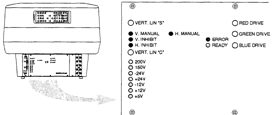
Figure 3-4. Rear Panel LEDs
