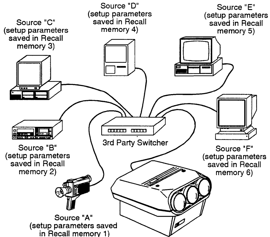
Figure 3-8. An Installation using the ASR Feature
