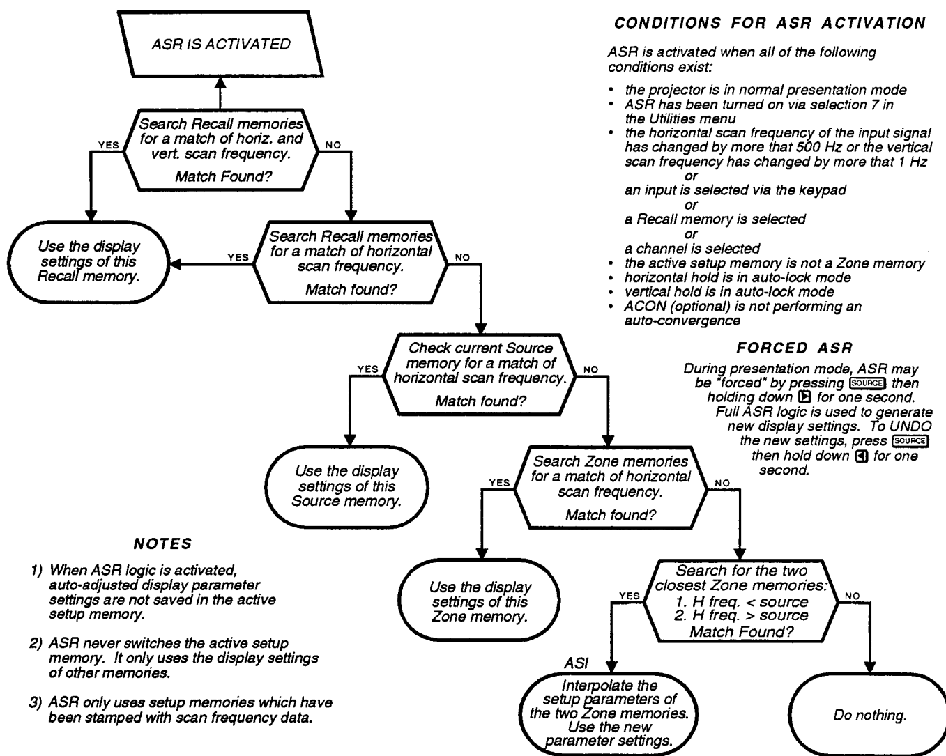
Figure C-1. ASR Logic Diagram
