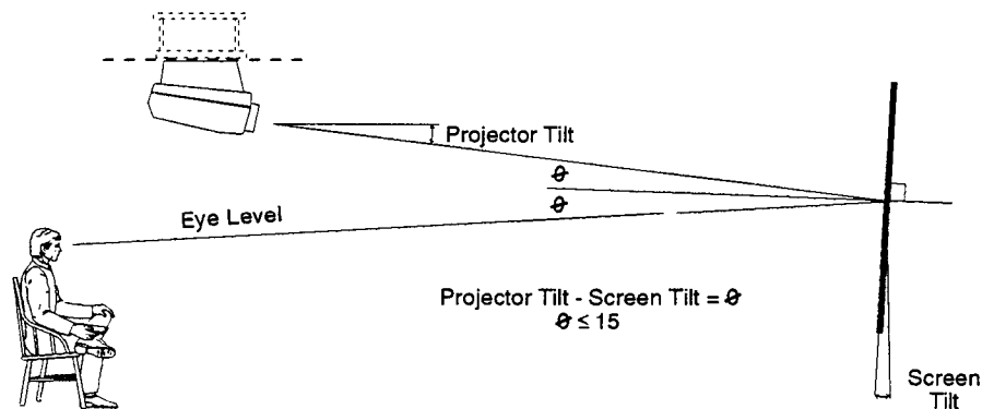
Figure 2-9. Ceiling Mount Installation
