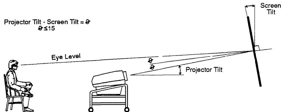
Figure 2-7. Floor Mount Installation
