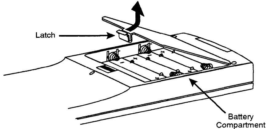
Figure 2-6. Battery Installation
