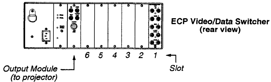
Figure 3-6. Switcher Slots
