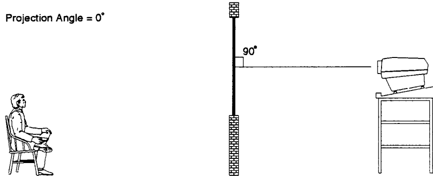
Figure 2-10. Optical Rear Screen Installation
