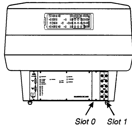
Figure 2-15. Projector Input Slots
